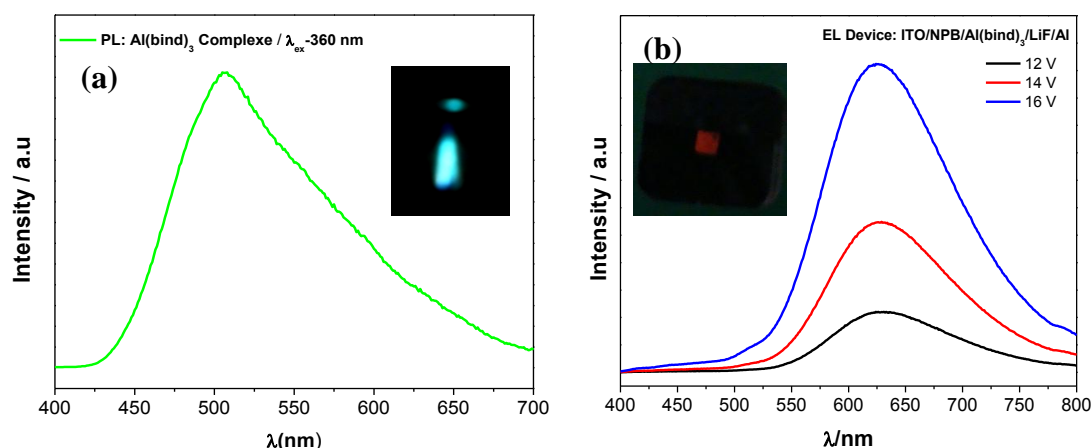
Fig. 1. Photo - and electroluminescence spectra recorded at room temperature (298 K), (a) PL spectra and picture of Al(bind) 3 complex with excitation at 360 nm (b) EL spectra picture of ITO/NPB/[Al(bind) 3 ]/LiF/Al device.
