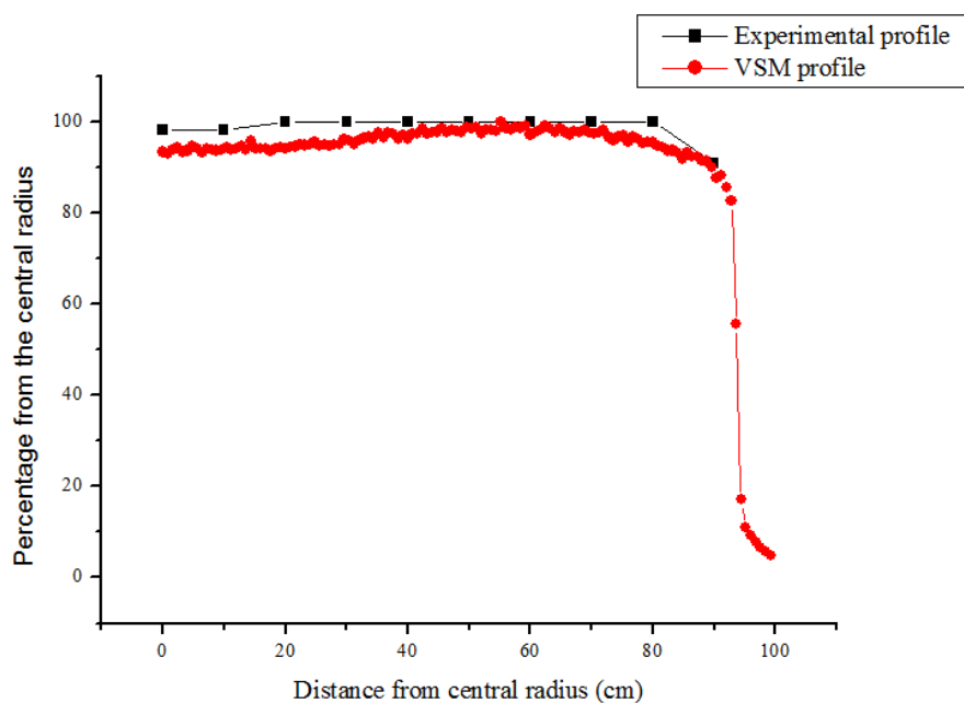
Figure 10: Profiles comparison between the experimental and VSM for a depth of 10.0 cm, 40\sqrt{2} \times 40\sqrt{2} cm 2 field.
