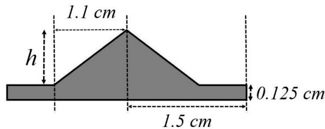
Figure 1: Scheme of the Virtual Flattening Filter (VFF).
