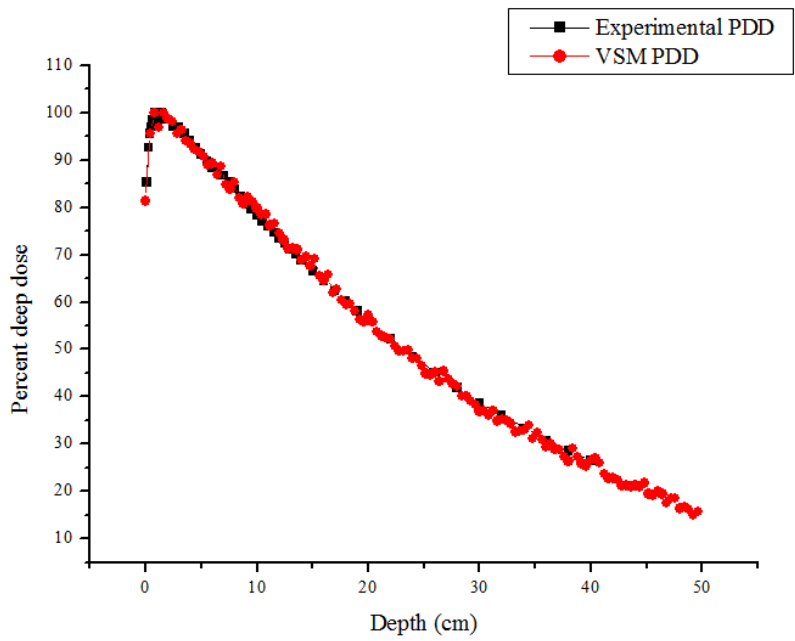
Figure 8: Comparison between experimental and VSM PDDs, 40\sqrt{2} \times 40\sqrt{2} cm 2 field.
