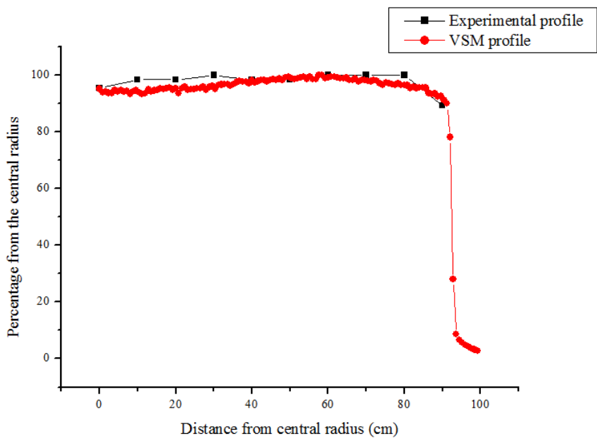
Figure 9: Profiles comparison between the experimental and VSM for a depth of 5.0 cm, 40\sqrt{2} \times 40\sqrt{2} cm 2 field.
