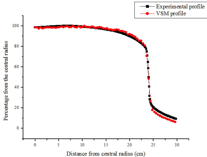
Figure 7: Profiles comparison between the experimental and VSM for a depth of 20.0 cm, 40 x 40 cm 2 field.
