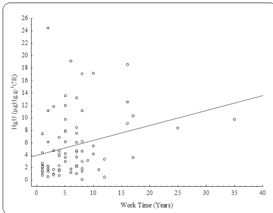
Figure 2 - Linear regression between the length of employment (years) and HgU concentration ( \mu\text{gHg}\cdot\text{g}^{-1}\text{CR} ).
