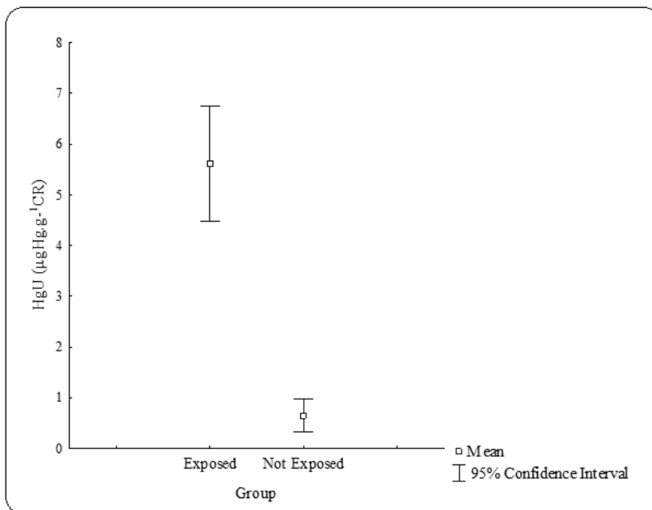
Figure 1 - Graphical representation of the mean HgU concentration in the exposed and unexposed groups.
