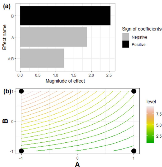
Fig. 4 (a) Pareto plots from the parameters calculated by the mathematical model for Y_2 (adsorption capacity of the composite, \text{mg g}^{-1} ); (b) contour plot of actual values for dosage ( A , \text{g L}^{-1} ) and [^{135}\text{Cs}]_0 ( B , \text{mg L}^{-1} ). Levels are predictions for Y_2 ( \text{mg g}^{-1} ).
