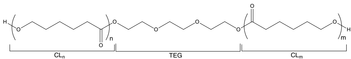
(a) Chemical structure of the synthesized PCL diol
